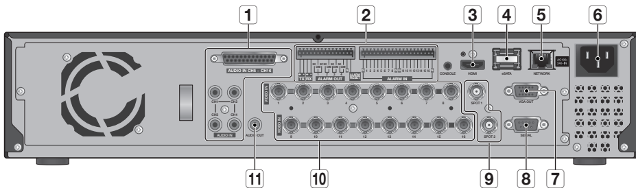
SRD-1653D/1673D
