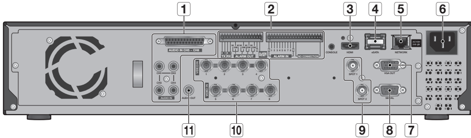
SRD-873D
